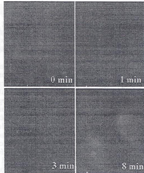
Fig. 1 UVA-induced modifications of CHO autofluorescence.
